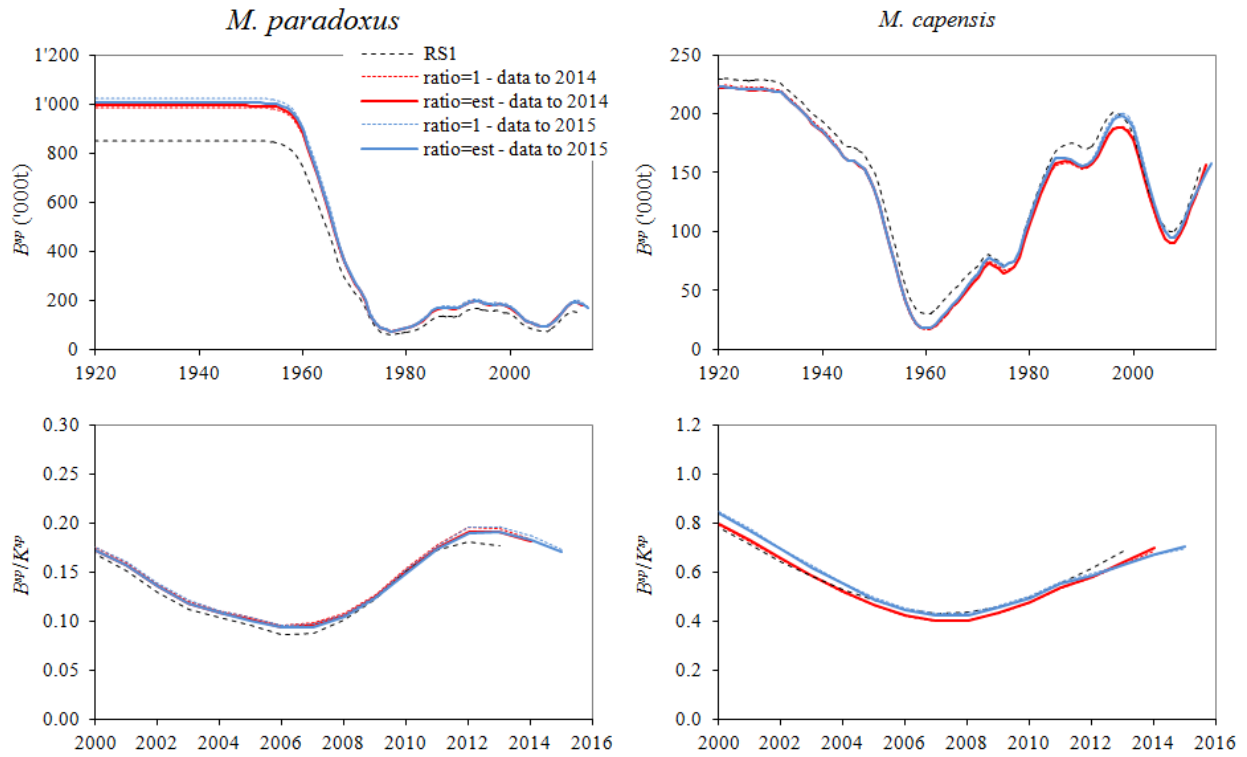
Figure 1: Spawning biomass trajectories (in absolute terms, top row, and relative to pre-exploitation level, bottom row) for the five cases for M. paradoxus (LHS) and M. capensis (RHS).
