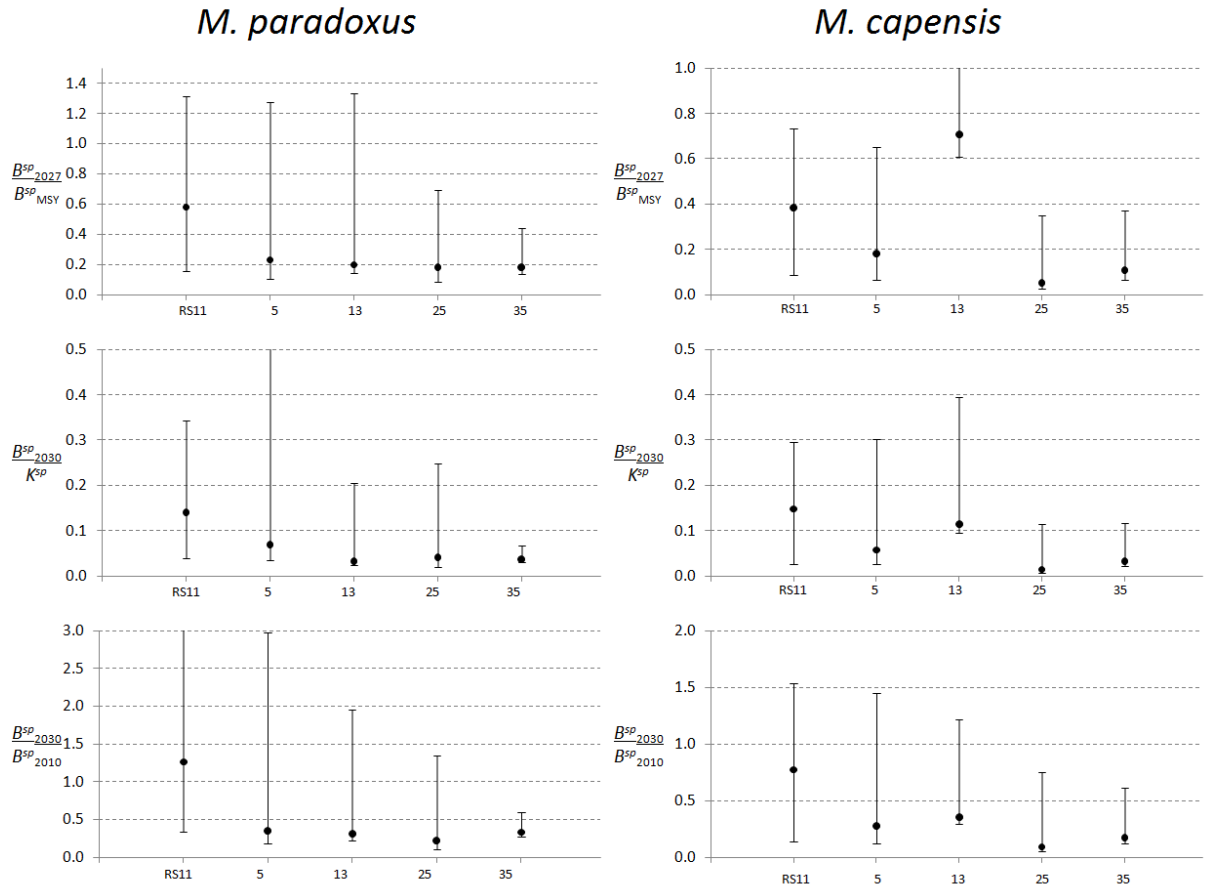
Fig. App.A.2: Three performance statistics ( B_{2027}^{sp} / B_{MSY}^{sp} , B_{2030}^{sp} / K^{sp} and B_{2030}^{sp} / B_{2010}^{sp} , in terms of female biomass only) for M. paradoxus and M. capensis for RS11 and four robustness tests based on this OM under a projected constant catch of 150 000t .
