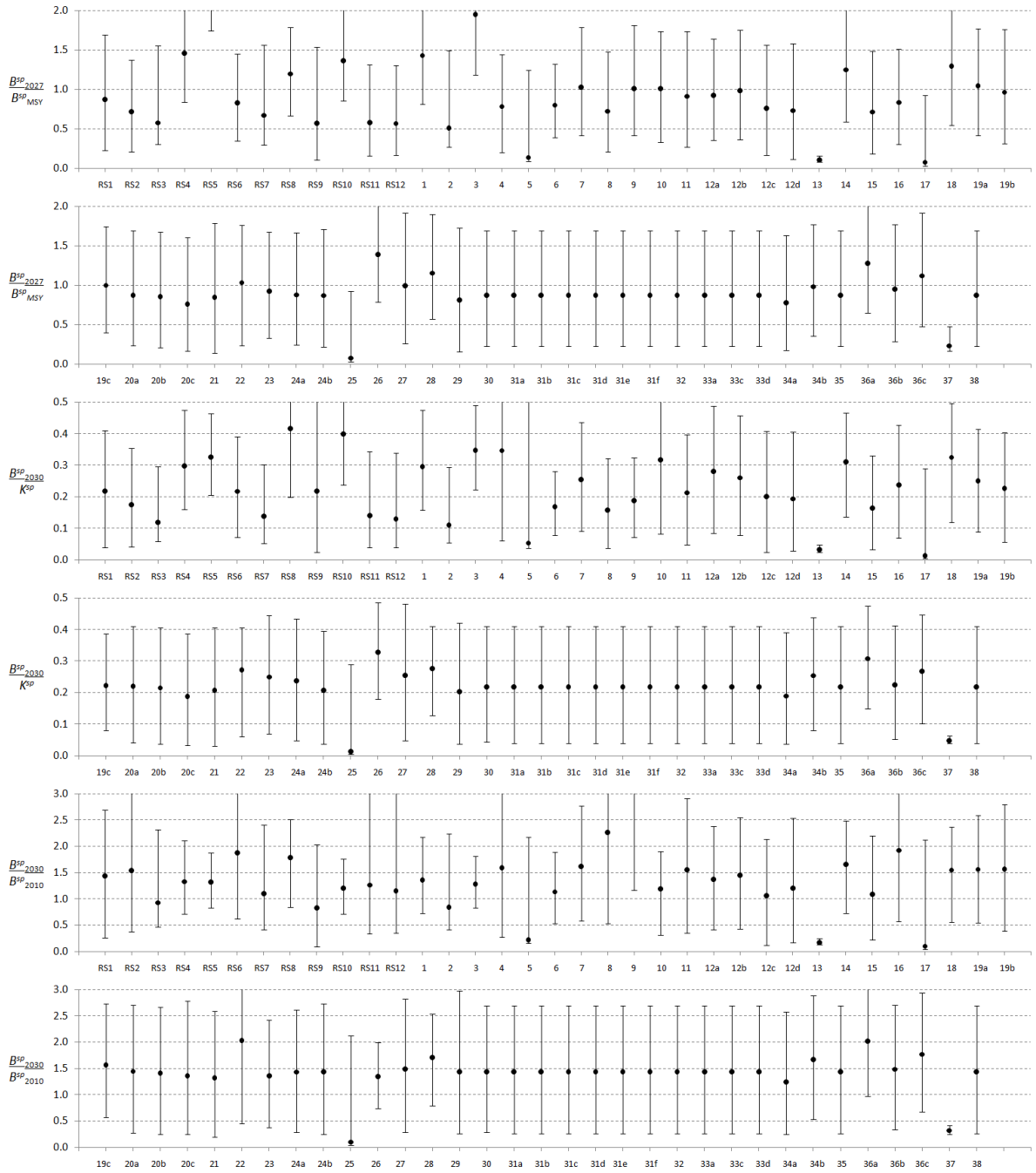
Fig. App.A.1a: Three performance statistics ( B_{2027}^{sp} / B_{MSY}^{sp} , B_{2030}^{sp} / K^{sp} and B_{2030}^{sp} / B_{2010}^{sp} , in terms of female biomass only) for M. paradoxus for the full set of RS and robustness tests under a projected constant catch of 150 000t . In some instance, the statistics are outside the area covered by the plot.
