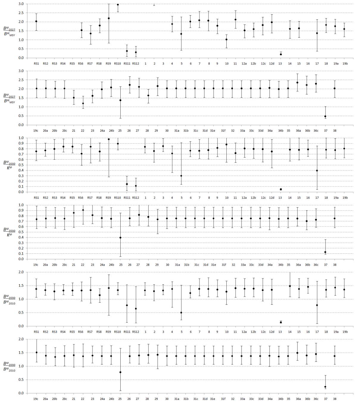
Fig. App.A.1b: Three performance statistics ( B_{2027}^{SP} / B_{MSY}^{SP} , B_{2030}^{SP} / K^{SP} and B_{2030}^{SP} / B_{2010}^{SP} , in terms of female biomass only) for M. capensis for the full set of RS and robustness tests under a projected constant catch of 150 000t . In some instance, the statistics are outside the area covered by the plot.
